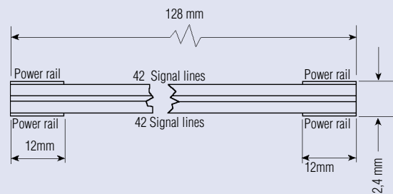
Multilayer Microbus backplanes
